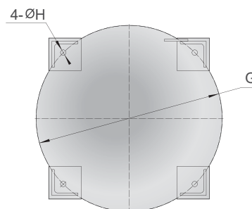
Mounting arrangement
