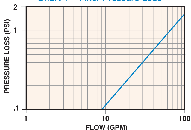
Chart 1 – Filter Pressure Loss
